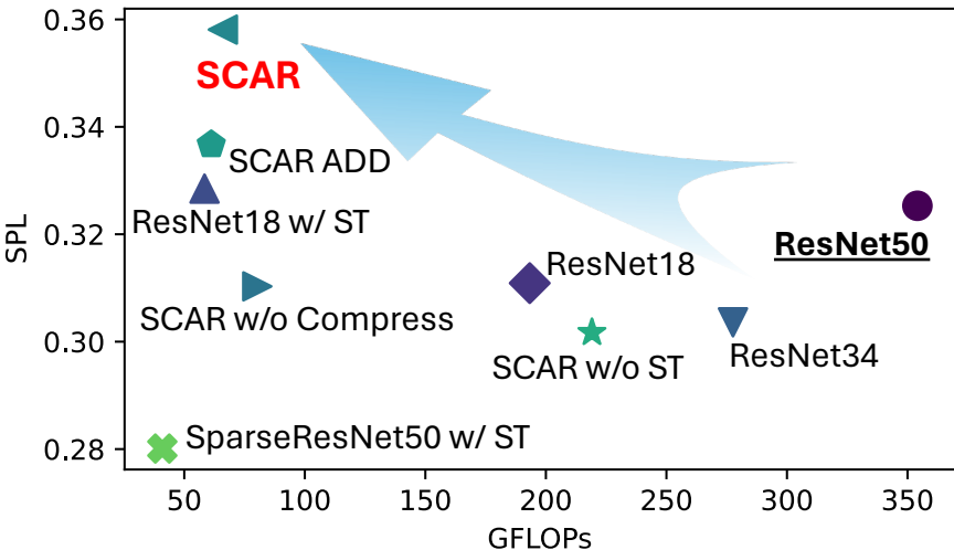
GFLOPs vs. SPL
